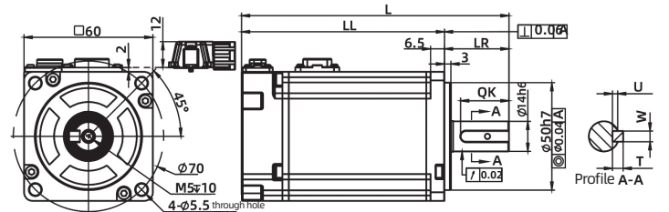
60mm flange
