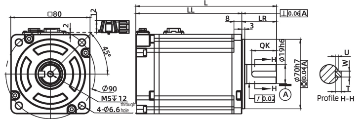
80mm flange
