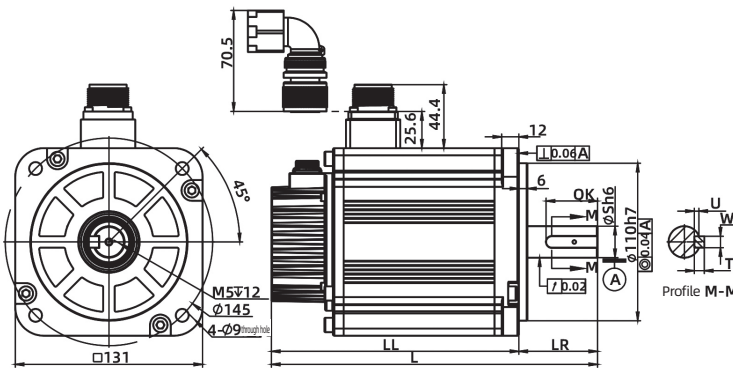
130mm flange
